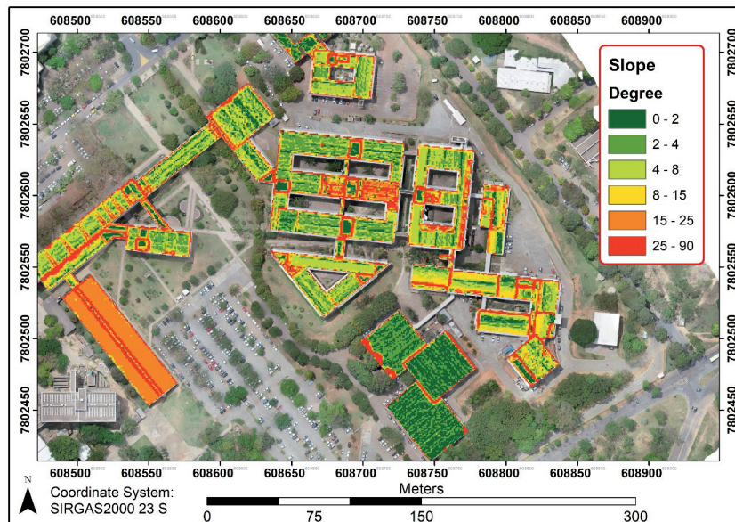
Figure 5 | Slope of the roofs of EE-IGC-UFGM.
